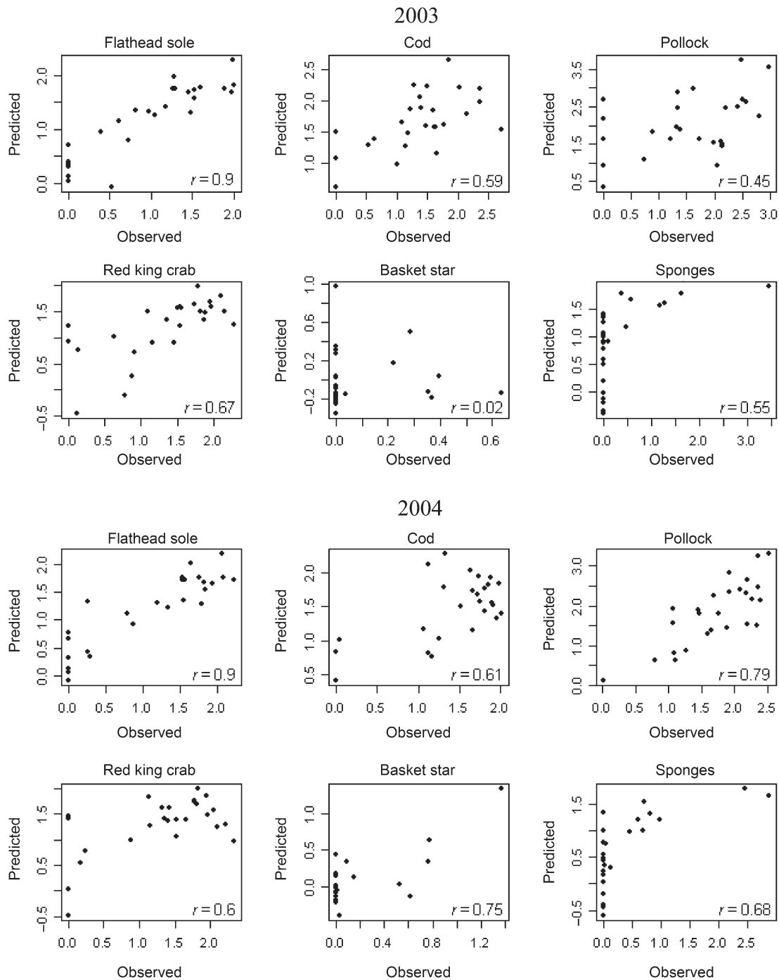
Figure 5. Predicted abundance (log-transformed \text{kg ha}^{-1} ) for 2003 and 2004 using best MLR models built with 2002 data (Table 2) vs. observed abundance for those years.
