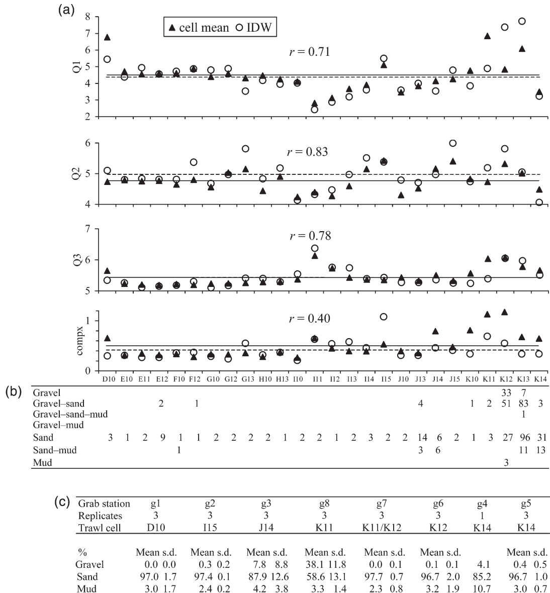
Figure 4. (a) Comparison of two methods (IDW and cell mean) for assigning a summary value of an acoustic variable (y-axis) to a trawl-survey cell (x-axis). For each acoustic variable, the cell values are plotted by method, with the mean of all cell values indicated (cell mean, solid line; IDW, dotted line; means generated by the two methods for Q3-values are so close that the lines overlap). The correlation ( r ) between the means calculated by each method is given. (b) The number of historical samples in each of seven “low-resolution” sediment classes in each trawl-survey cell. (c) Percentages (mean and standard deviation) of three sediment types in trawl-survey cells determined from grab samples in this survey (Figures 1 and 2); station g4 has only one sample (replicates = 1) and therefore no statistics; station g7 straddled trawl cells K11 and K12.
