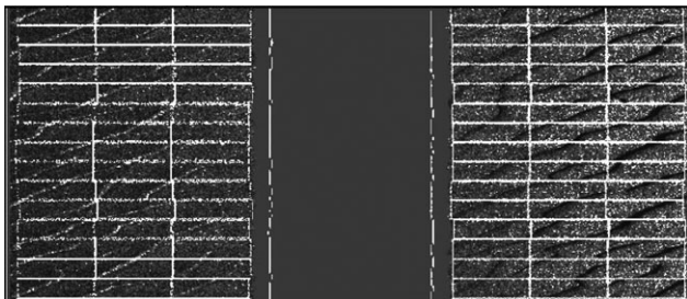
Figure 3. Sidescan-sonar image of seabed in QTC SIDEVIEW image viewer with rectangular patches placed over high quality data areas to either side of the data mask at the centre. The mask removes noise artefacts from the water column.
